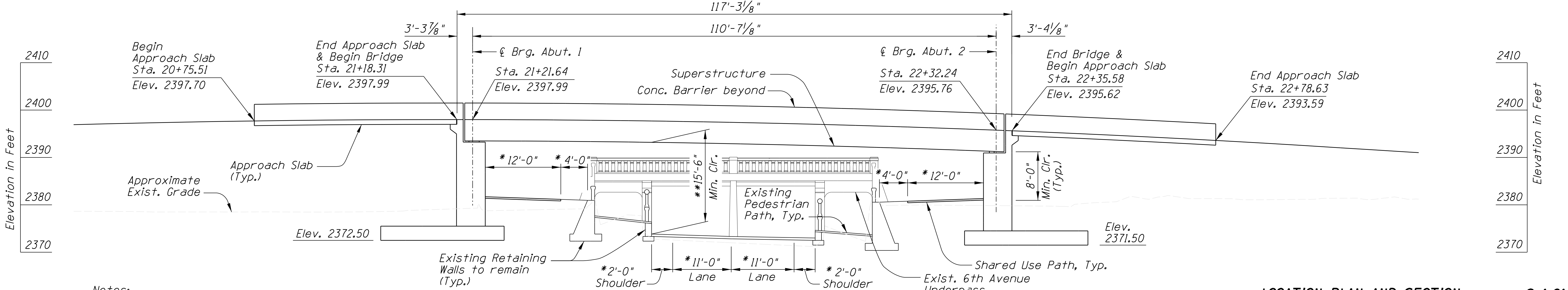
SECTION AT CONSTR. 1"=10'-0"
